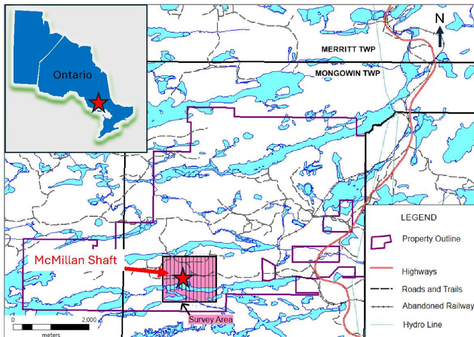
Figure 13 - McMillan Geophysical Survey Area
