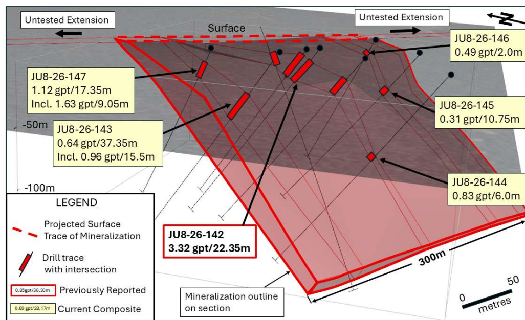
Figure 4 – 826 Zone gold mineralized envelope – looking east
