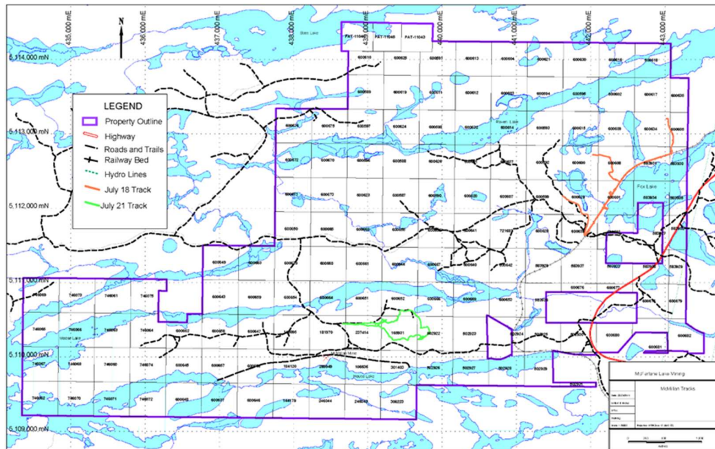
Figure 12 – Prospecting Tracks
