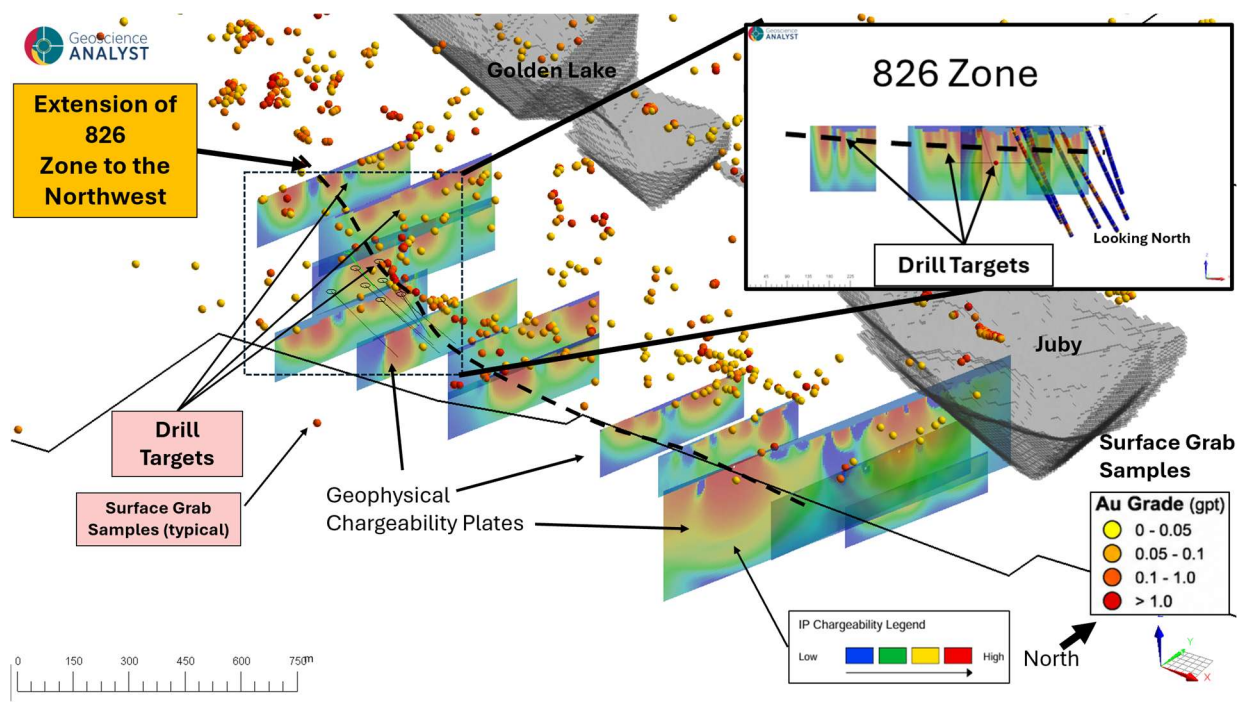
Figure 6 – 826 Zone – View of the 826 zone geophysical drill targets south of Golden Lake and Juby
