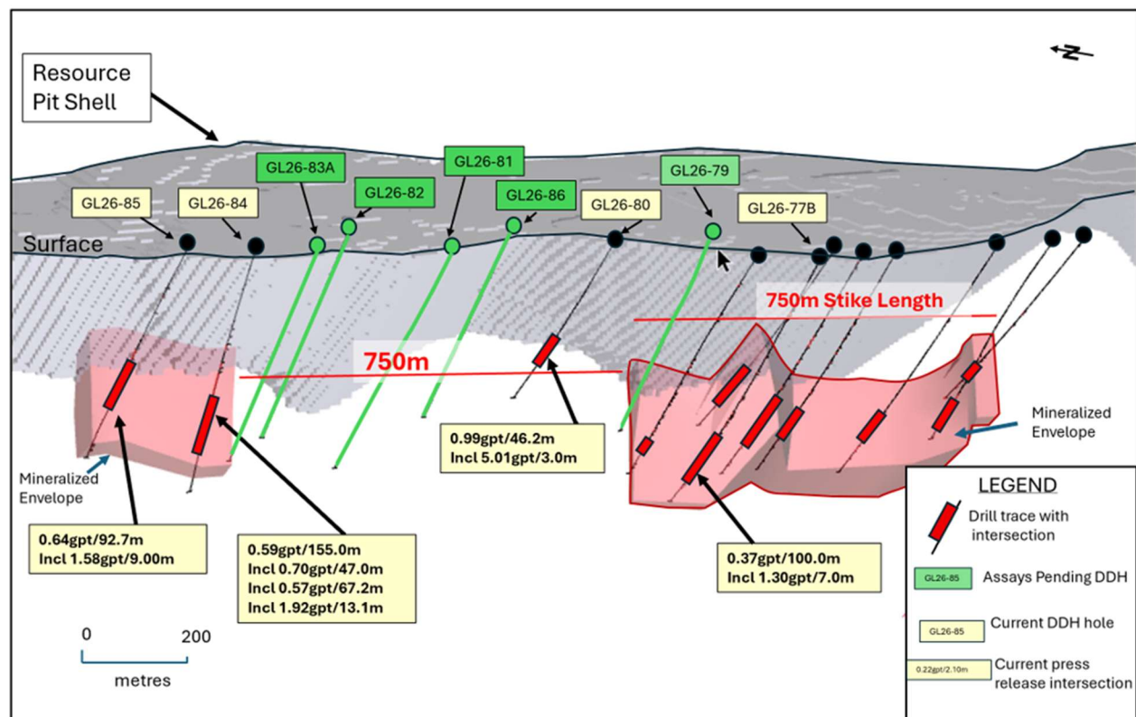
Figure 9 – Extension of mineralization - Golden Lake Deposit, looking north
