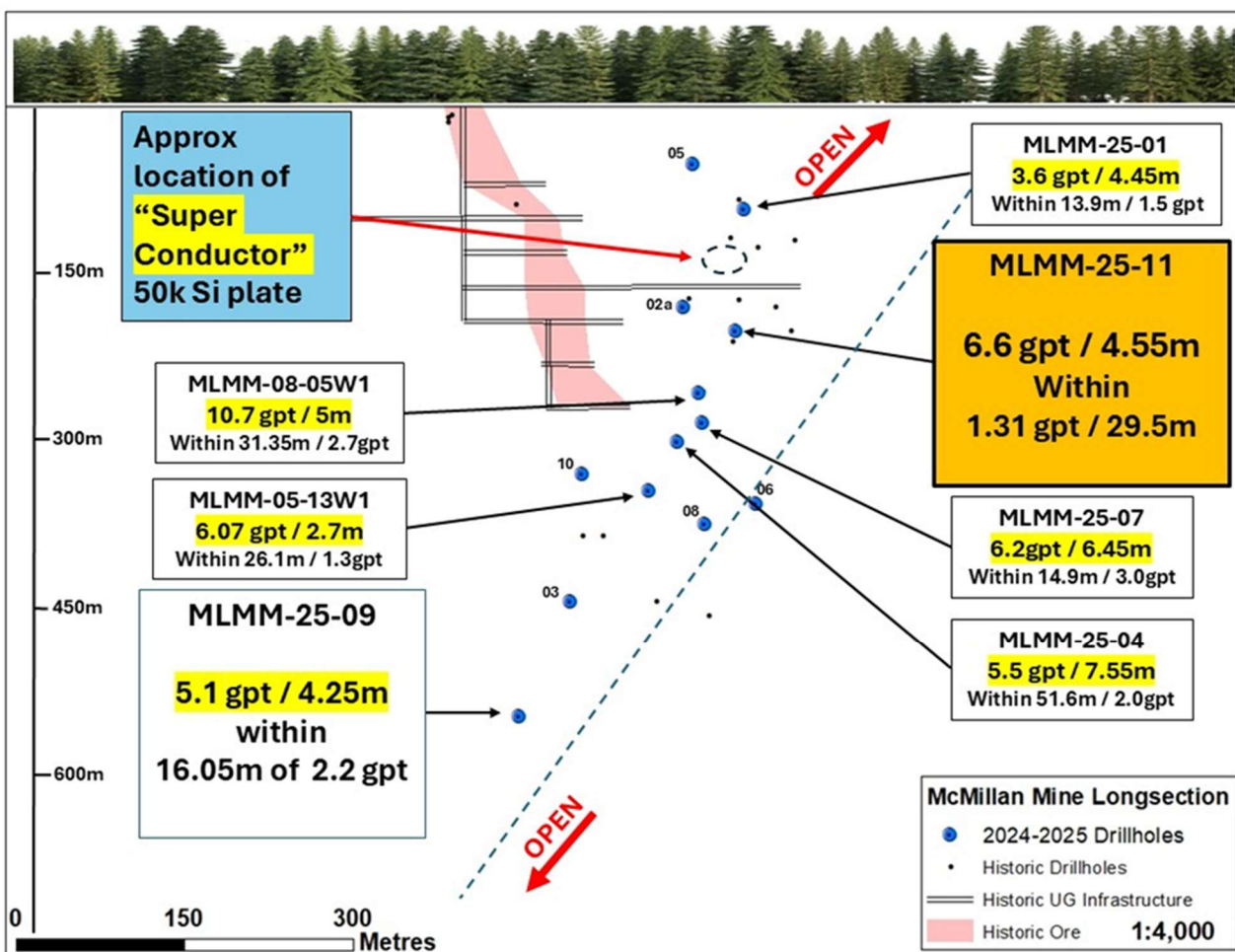
Figure 14 – McMillan Mine Longitudinal Section Looking North – Historic Gold Intercepts and Mine Workings
