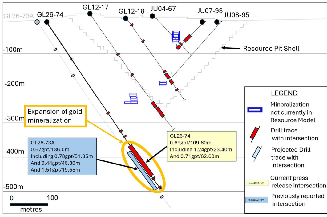
Figure 8 – Golden Lake intersection - drillhole GL26-74 – Section looking northwest
