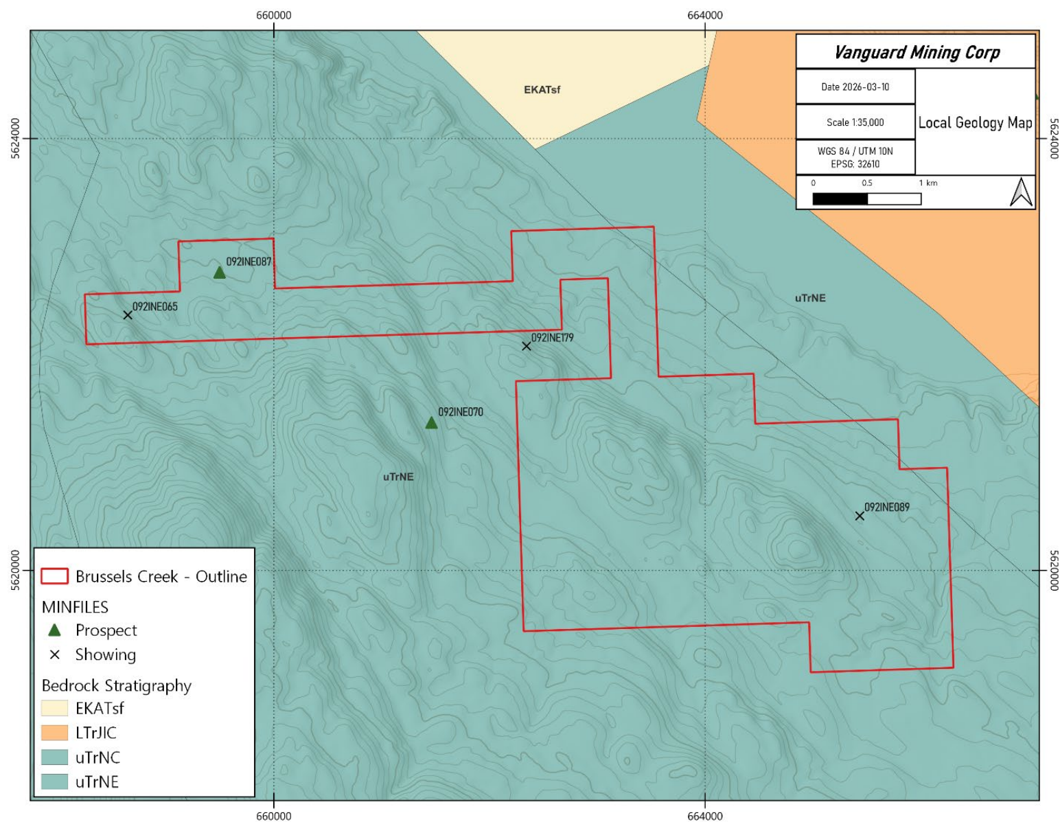
Figure 7-4: Local Geology.
