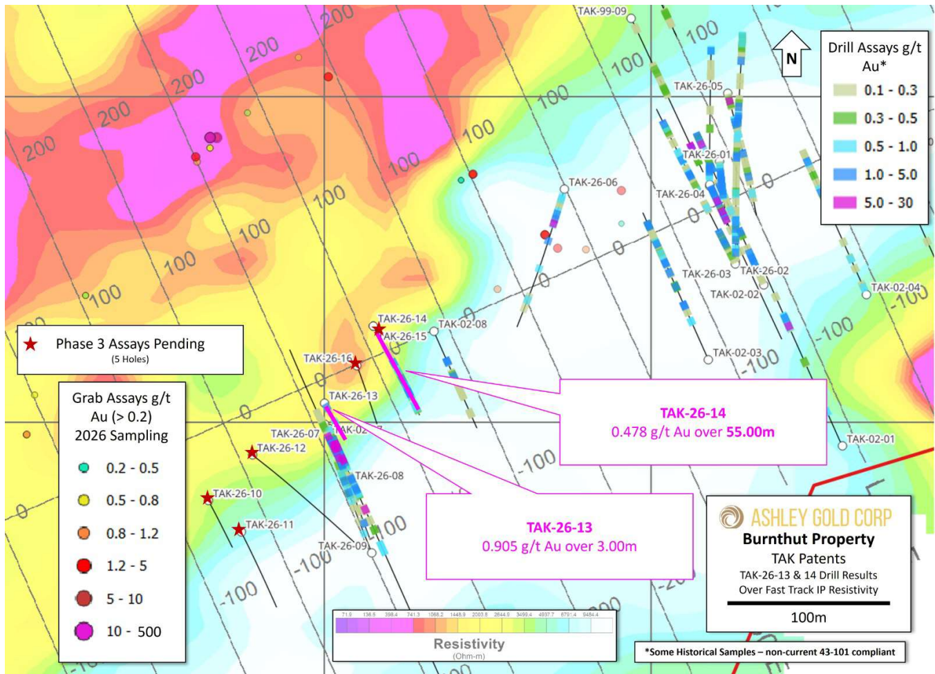
Figure 1: Tak Plan View
