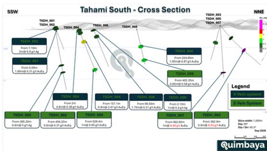
Figure 1. Tahami South cross section, 1,000 meter slice, dip direction 95.5 degrees, showing Phase 1 drill holes and selected intercepts. Selected intervals are shown and are not necessarily representative of mineralization on the property. Quimbaya Gold Inc., September 2026.
