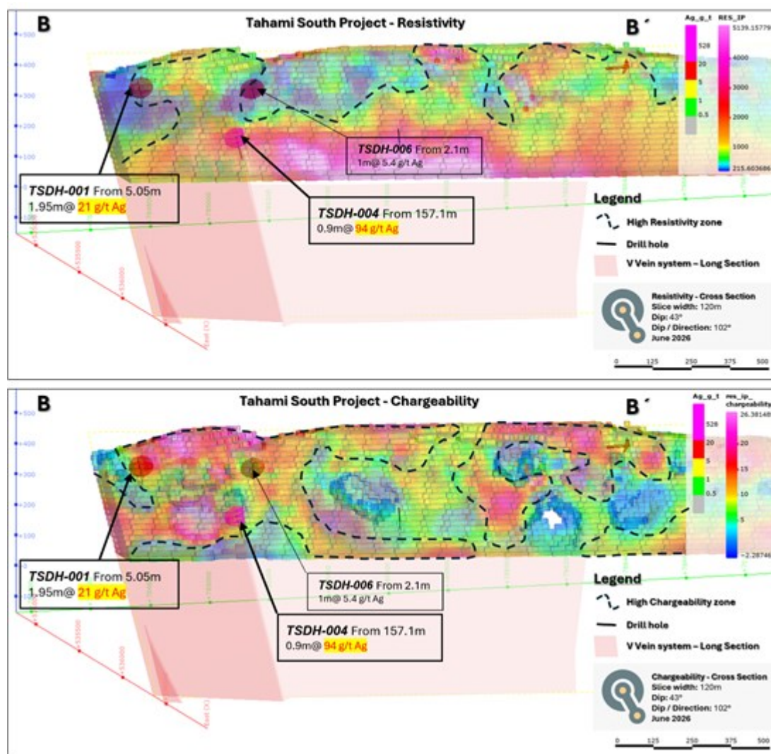
Figure 3. B - B'Long section of Resistivity (up) and Chargeability (down) derived from the 2026 IP 3D survey. Moderate to high resistivity value are interpreted as resistive silicified zones (quartz veins) or structural feeder zone. Elevated chargeability values reflect zones of increased sulphide content within the interpreted V Veins system and potential mineralized shoots.
